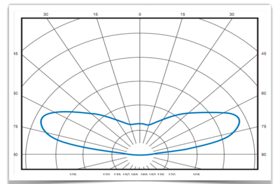
Light Distribution Graph
